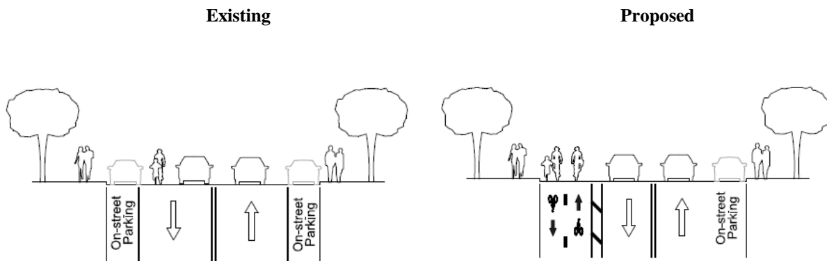
Figure 1 – Typical Cross Sections for Barton Hills Drive
